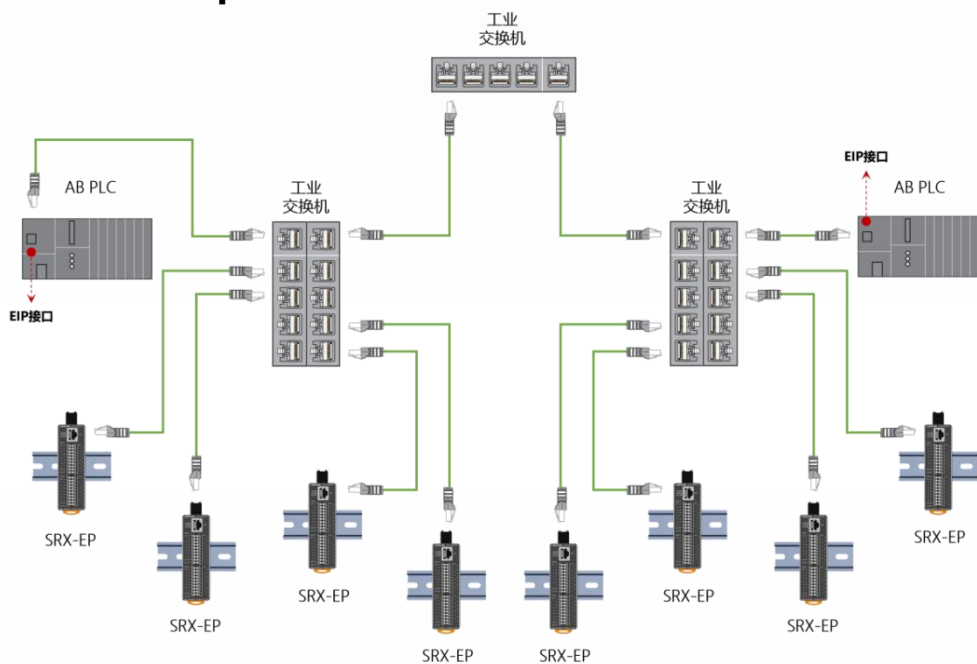
Figure 5-3 ETHERNET/IP Tree Network Topology Structure
