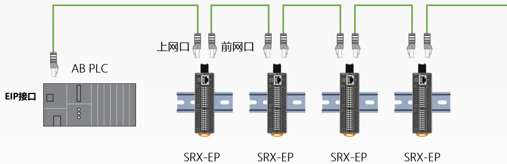
Figure 5-2 ETHERNET/IP Daisy Chain Network Topology Structure
