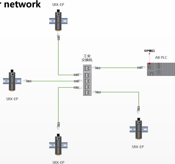
Figure 5-1 ETHERNET/IP Star Network Topology Structure
