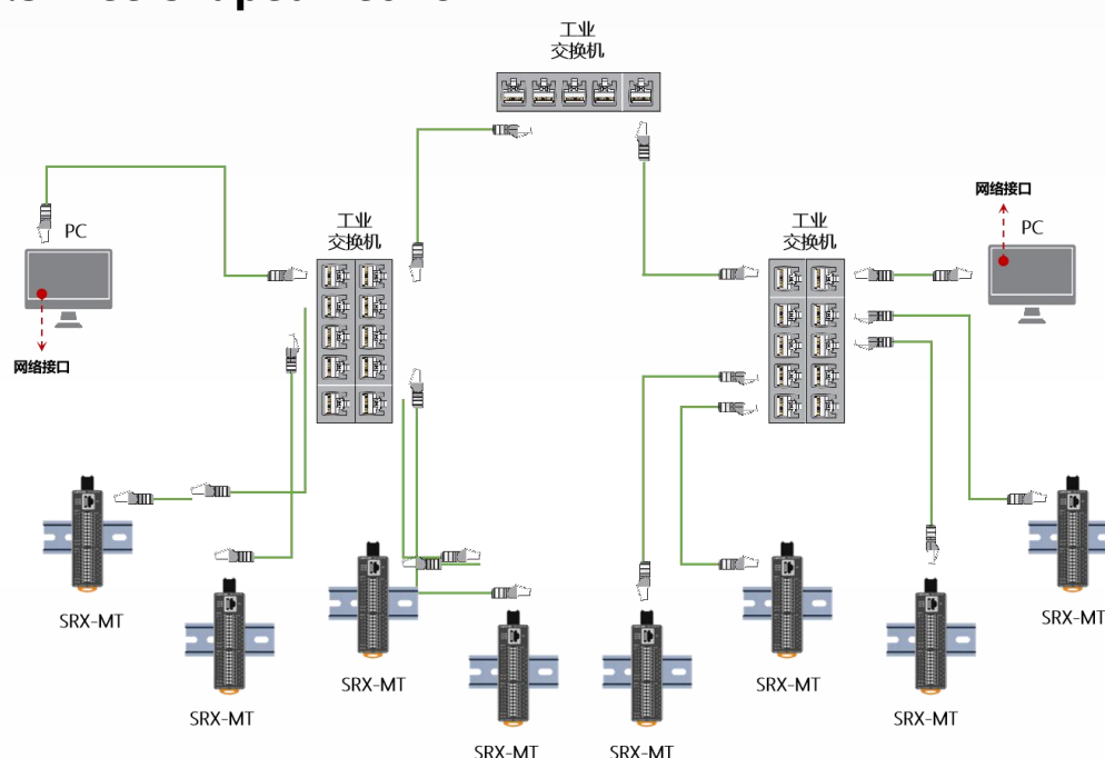
Figure 5-3 Modbus-TCP Tree Network Topology Structure
