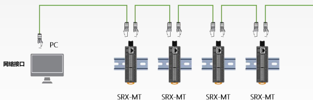
Figure 5-2 Modbus-TCP Daisy Chain Network Topology Structure
