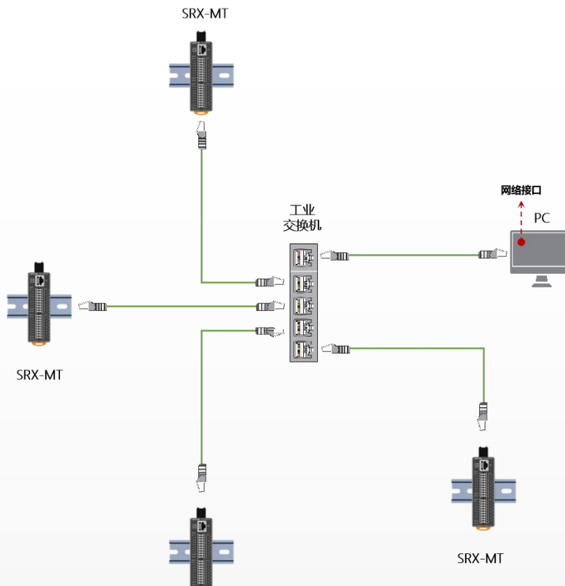
Figure 5-1 Modbus-TCP Star Network Topology Structure
