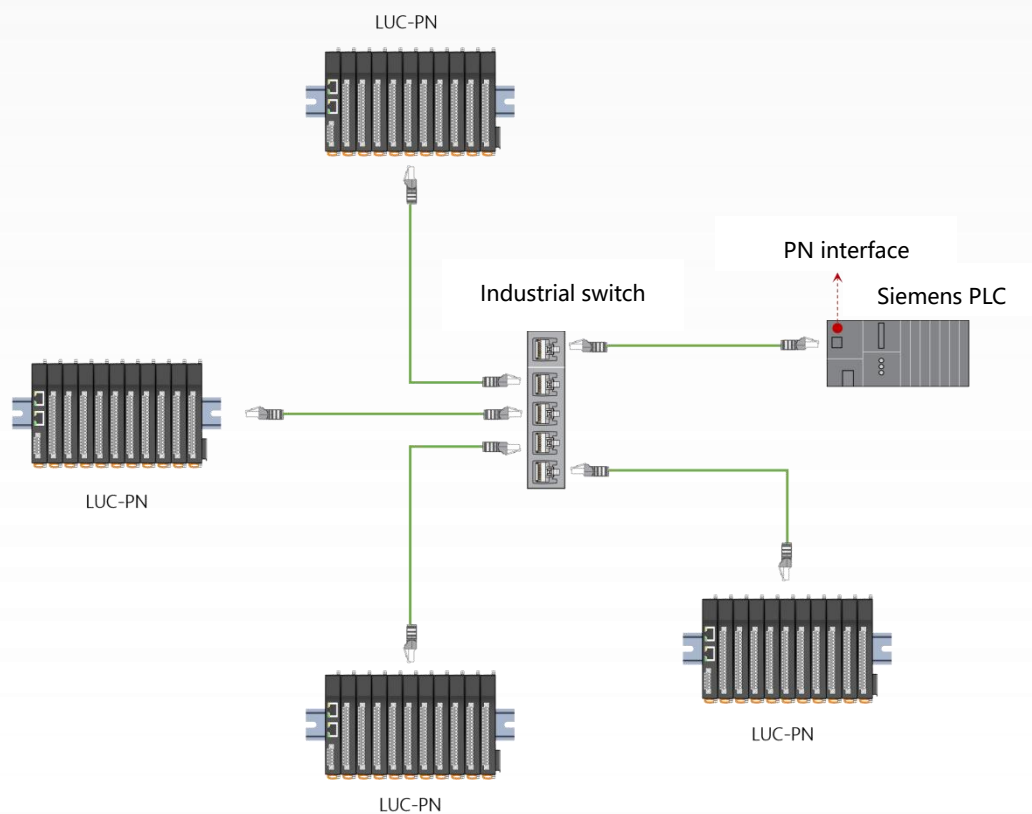
Figure 1-1 PROFINET Star Network Topology
