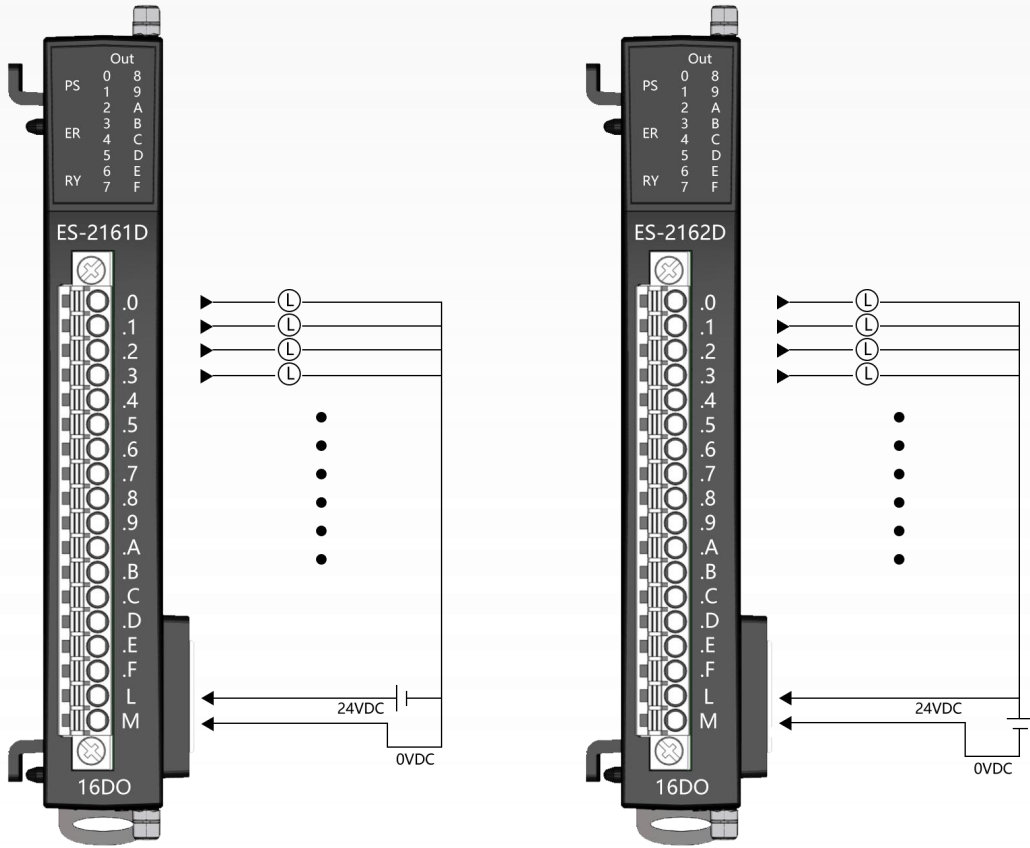
High level output wiring method (PNP) Low level output wiring method (NPN)
