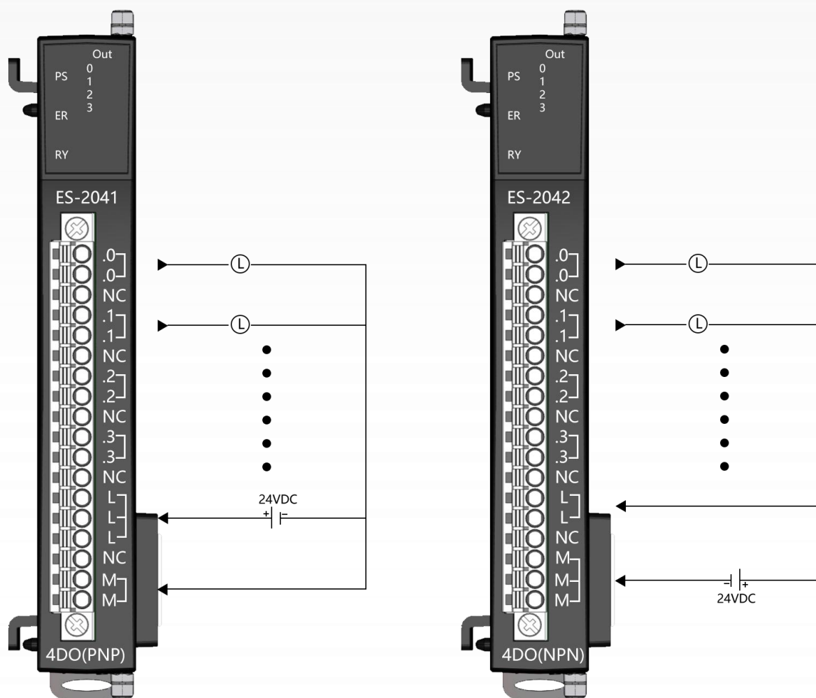
High-level output wiring method (PNP)
