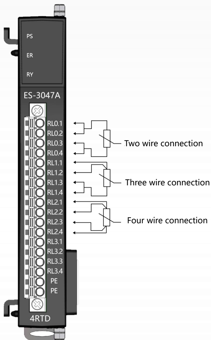
PT100 2-wire, 3-wire, 4-wire wiring diagrams
