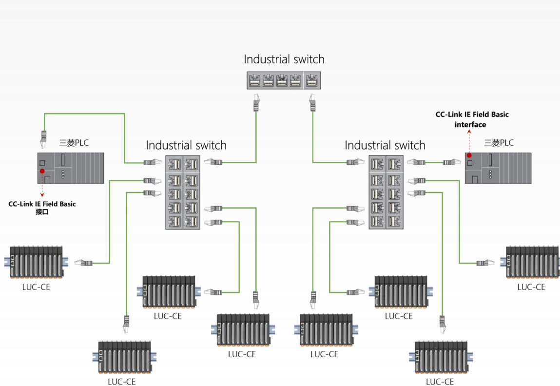
Figure 3-2 CC-Link IE Field Basic Tree Network Topology
