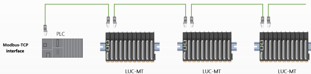
Figure 2-2 Modbus-TCP daisy chain topology
