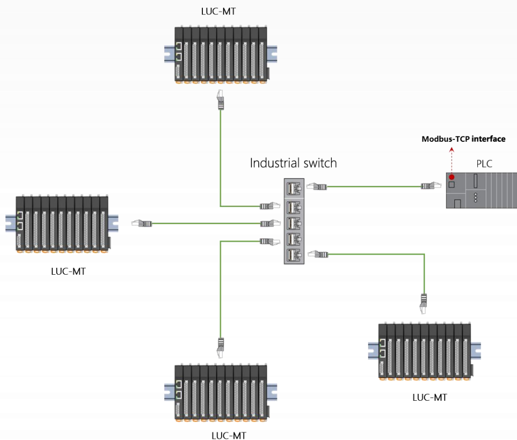
Figure 2-1 Modbus-TCP Star Network Topology
