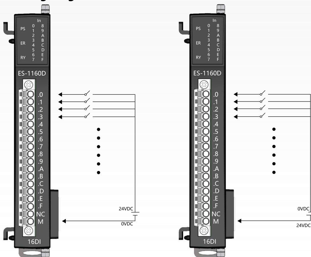
High-level input wiring method (PNP) Low-level input wiring method (NPN)
