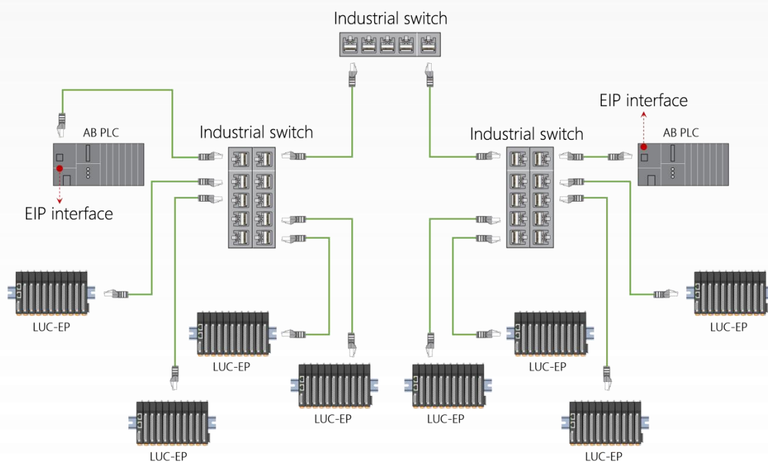
Figure 2-3 ETHERNET/IP Tree Network Topology
