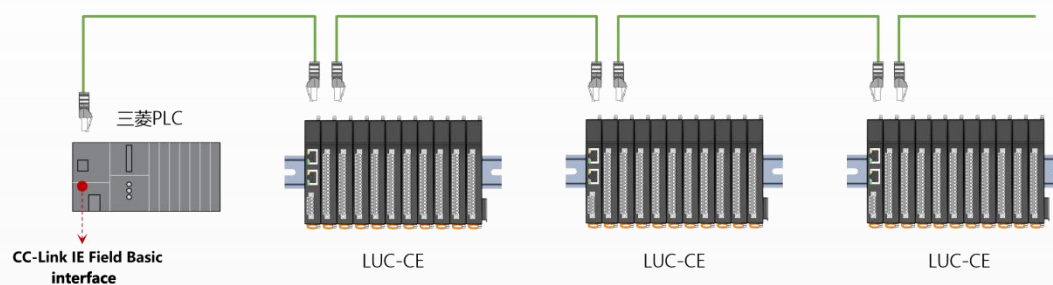
Figure 3-3 CC-Link IE Field Basic daisy chain topology
