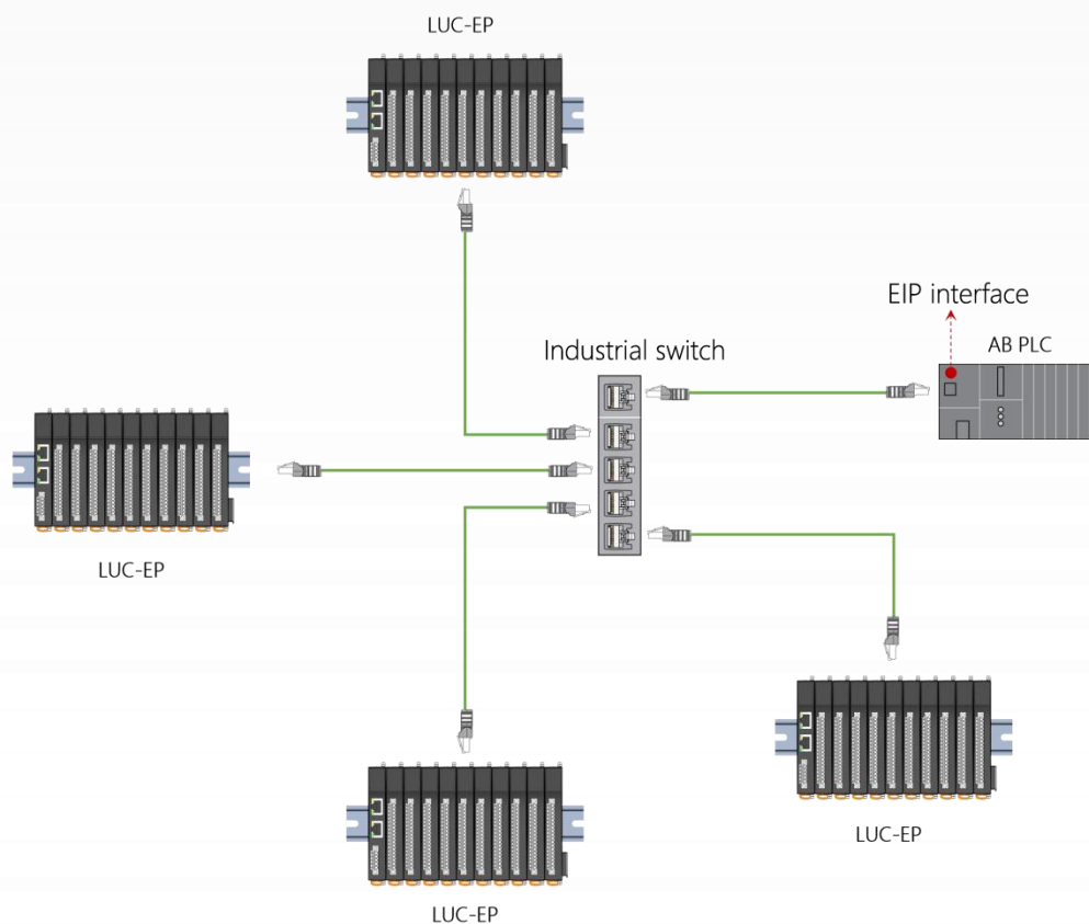
Figure 2-1 ETHERNET/IP Star Network Topology
