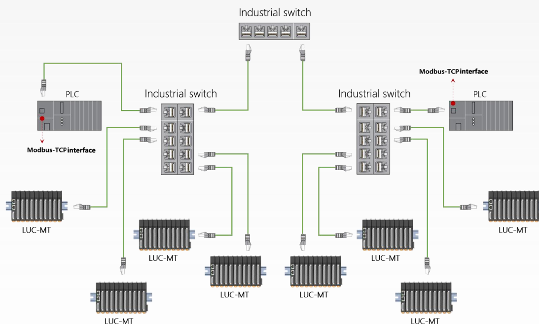
Figure 2-3 Modbus-TCP Tree Network Topology
