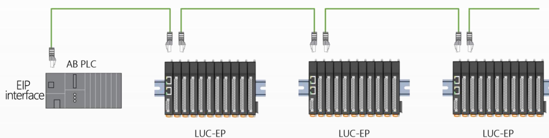
Figure 2-2 ETHERNET/IP daisy chain topology
