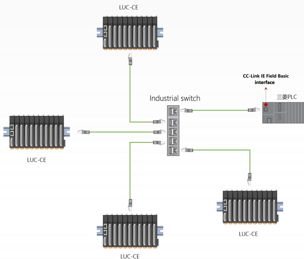
Figure 3-1 CC-Link IE Field Basic Star Network Topology
