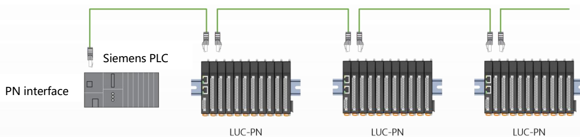
Figure 1-2 PROFINET daisy chain topology
