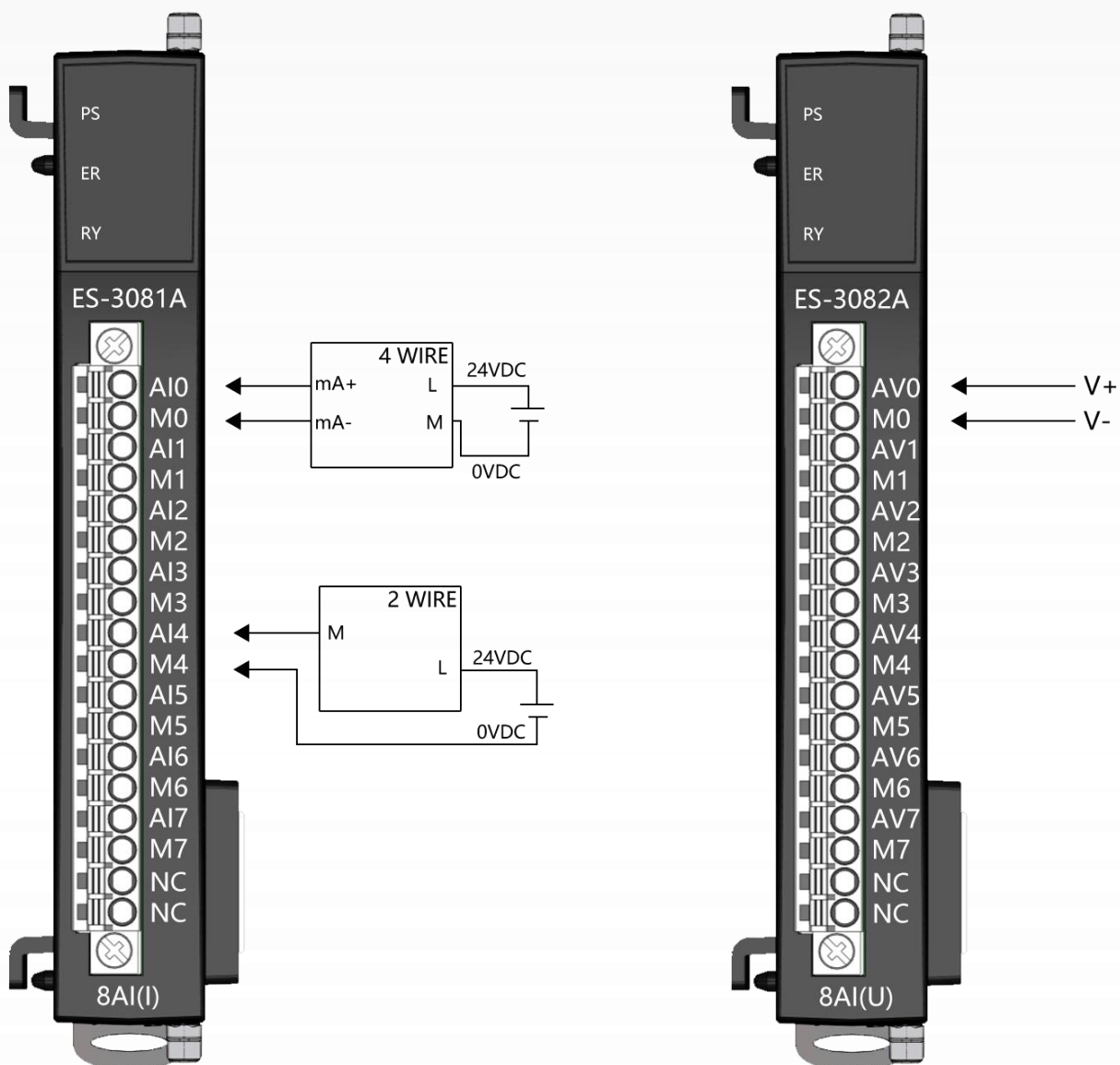
Analog current input wiring method Analog voltage input wiring method
